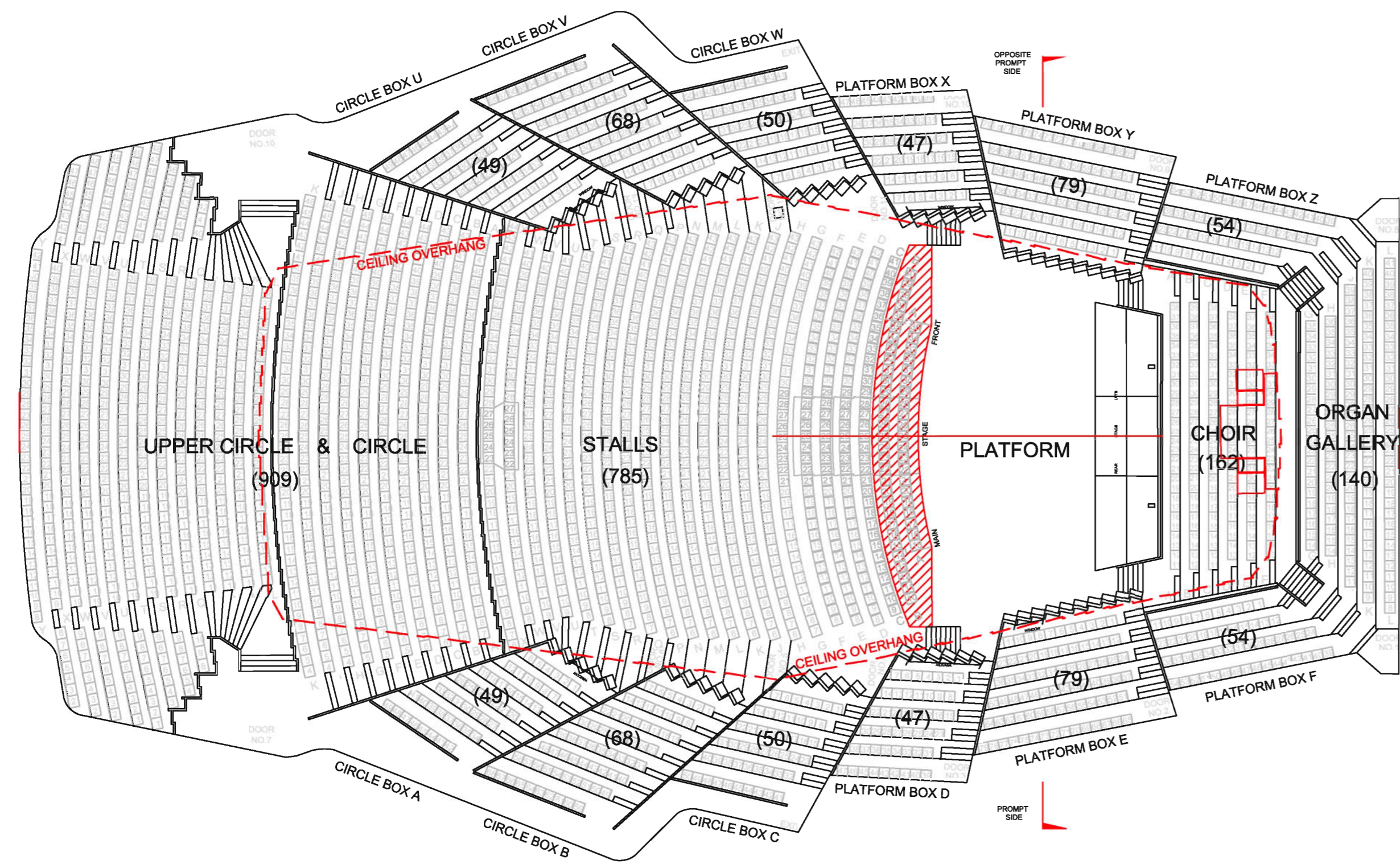
PLAN VIEW
