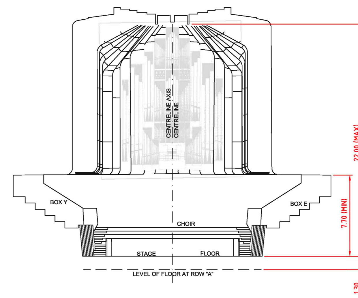
ORGAN ELEVATION
