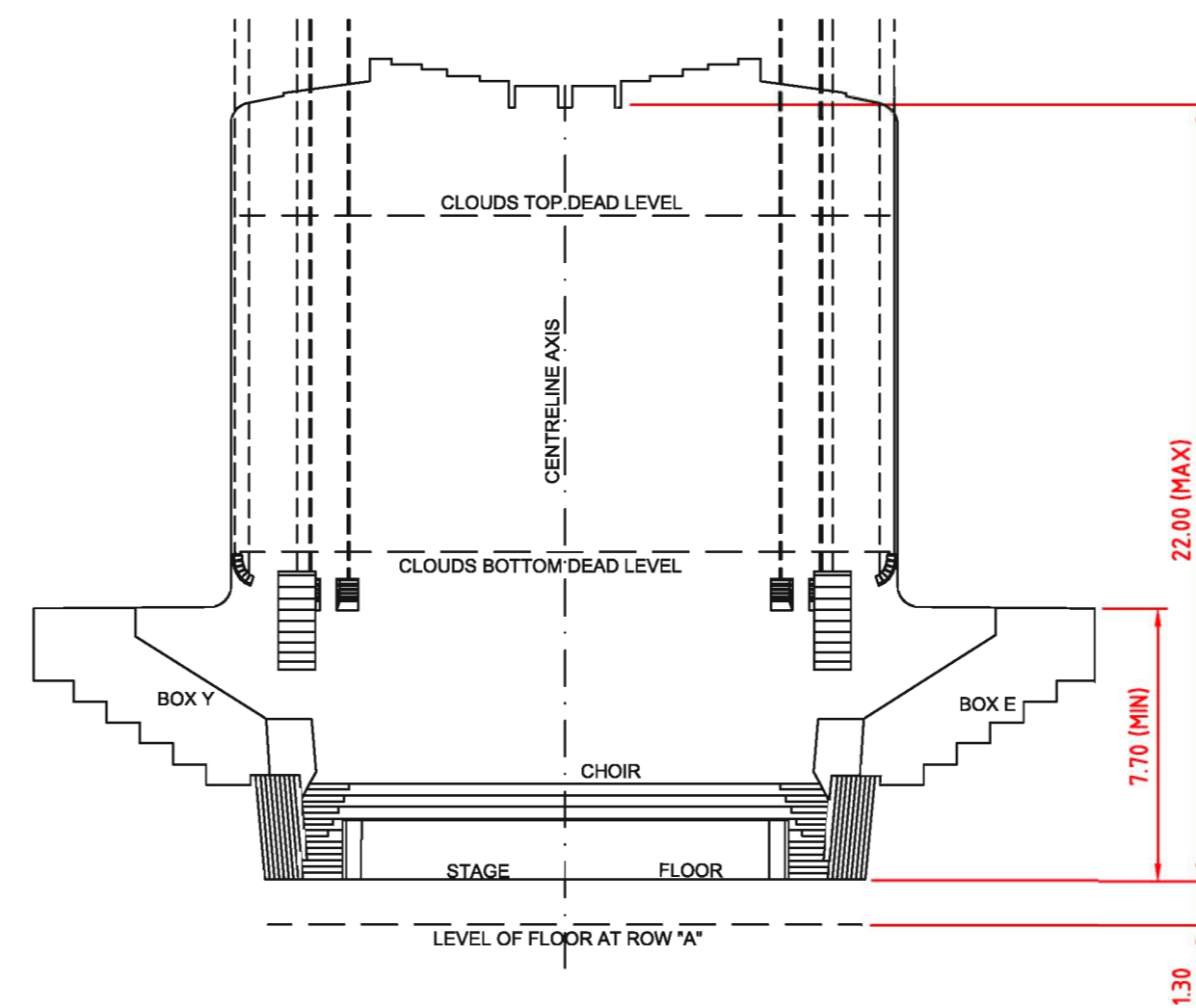
EAST-WEST SECTION
