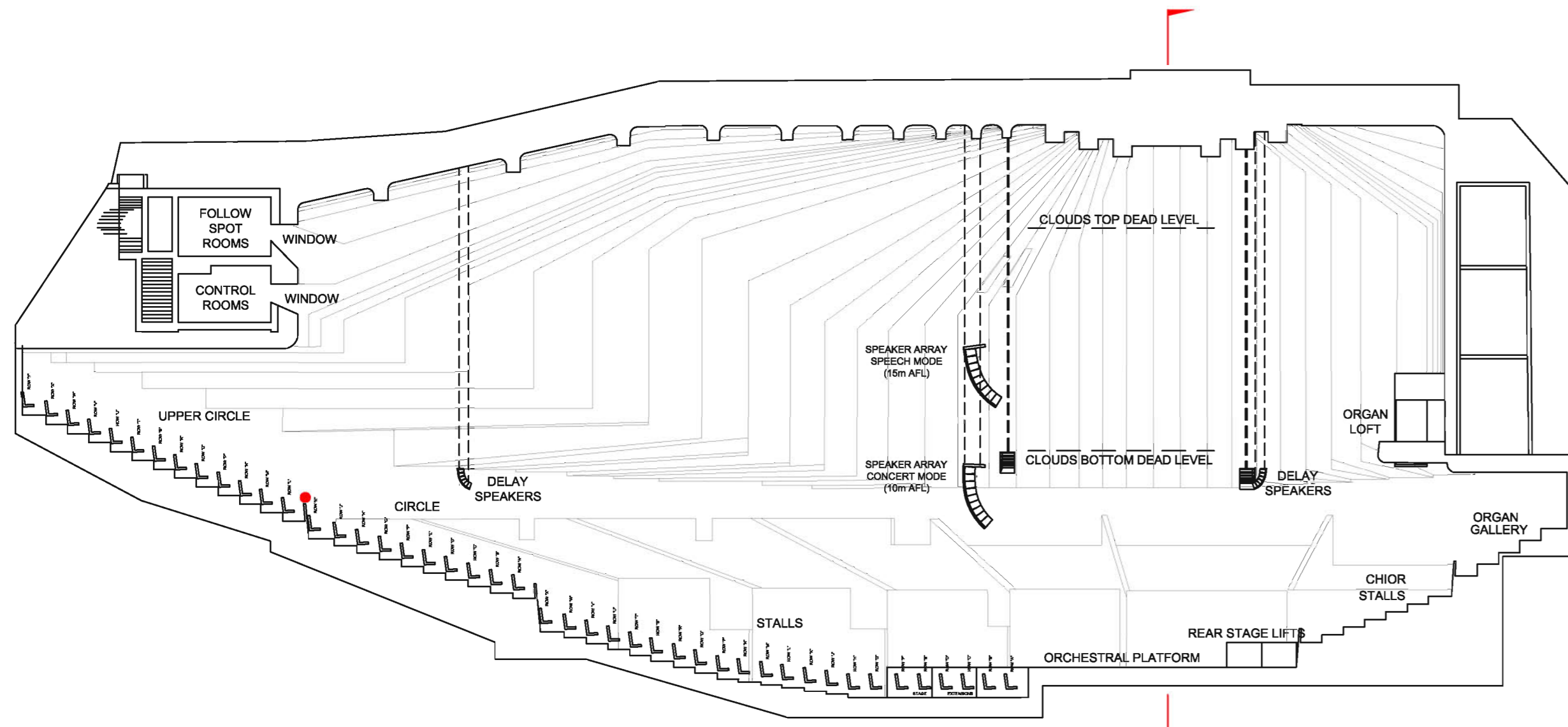
NORTH-SOUTH SECTION
